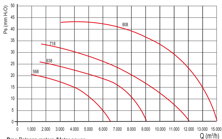
8 poli/poles (750 rpm) - trifase/three-phase
